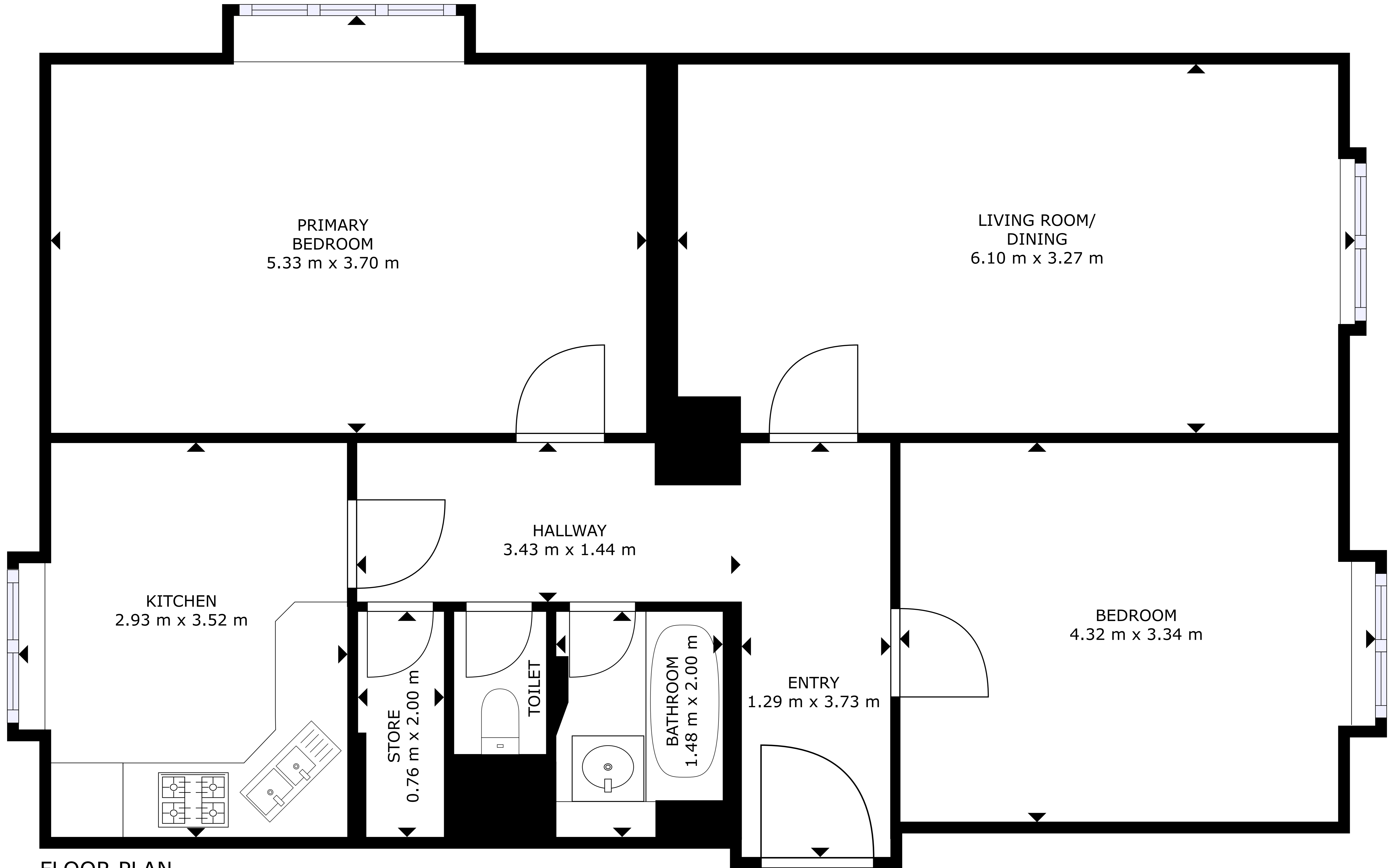
FLOOR PLAN
