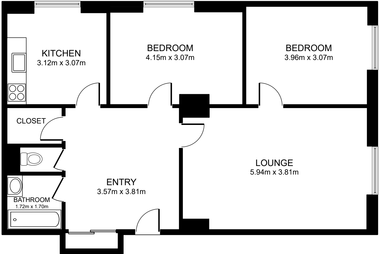
FLOOR PLAN FLOOR AREA 80.8 SQ.M. APPROX
